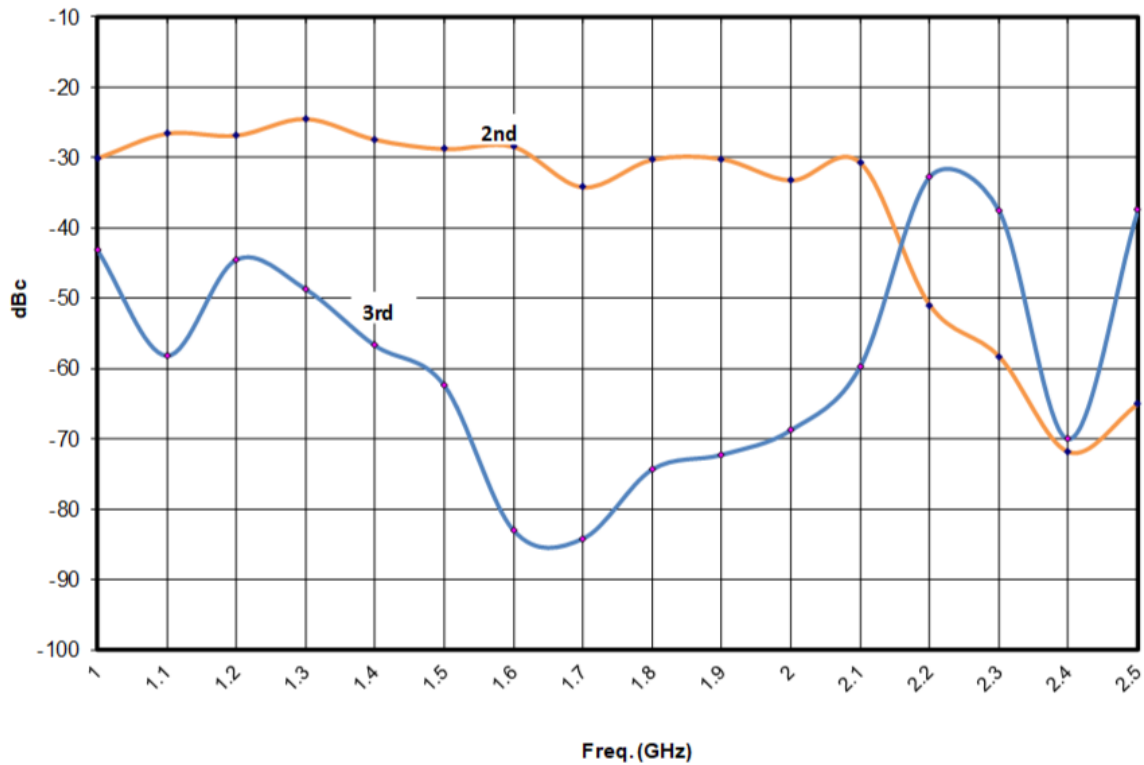
TYPICAL HARMONICS @ 750 WATTS
